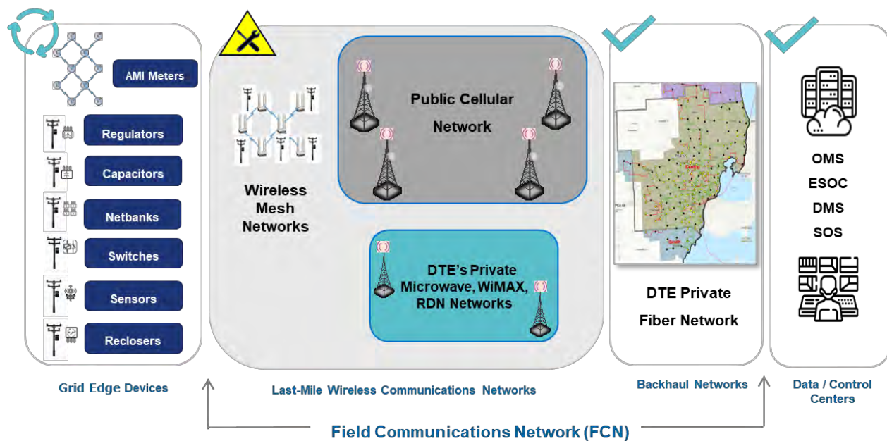
Exhibit 6.85 – DTE's Current FCN
