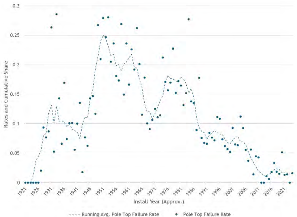
Figure 2-10: Pole Top Inspection Failure Rates
