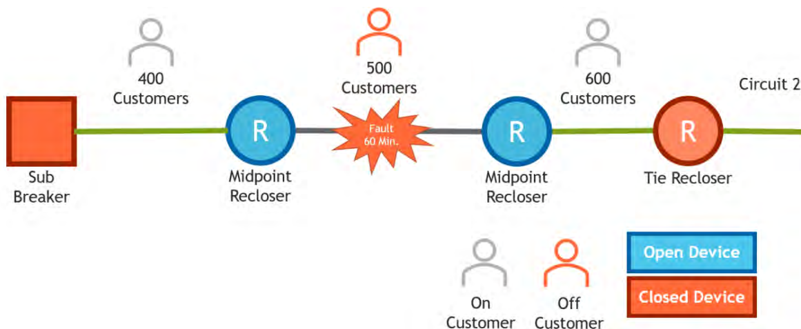
Figure 4-26: Simplified Diagram of Circuit with Automate Ties Scheme
