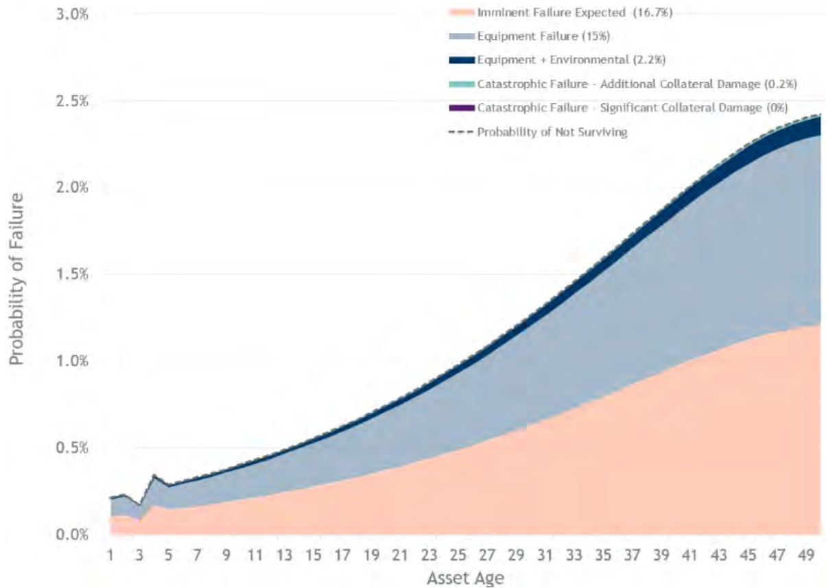
Figure 4-19: Investment Scenario Probability of Failure Profiles
