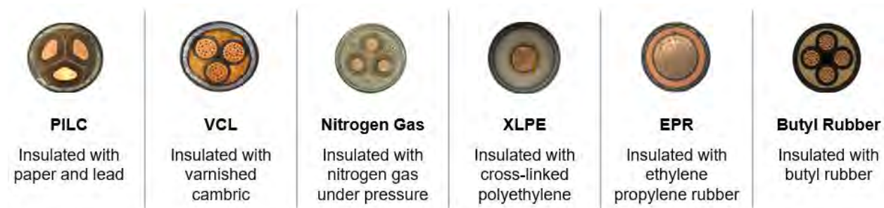
Exhibit 4.23 – Underground System Cable Types
