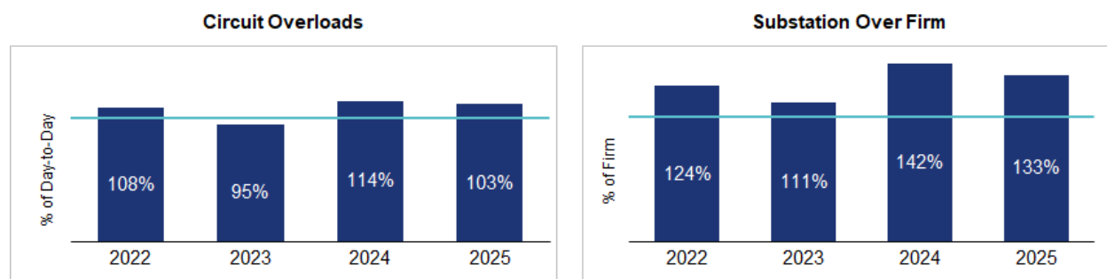
Exhibit 6.51 – Port Austin Loading Issues, 2022-2025
