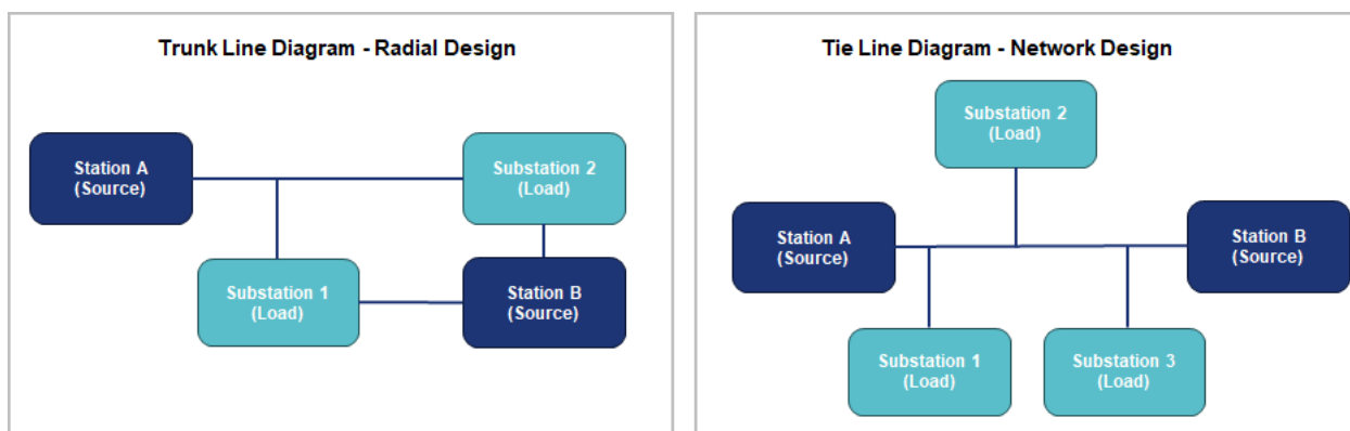
Exhibit 4.4 – Subtransmission Radial and Network Designs
