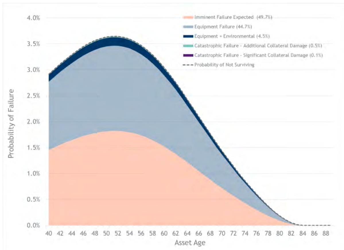
Figure 4-13: Failure Types and Probability of Failure for 40-Year-Old Oil Distribution Breaker
