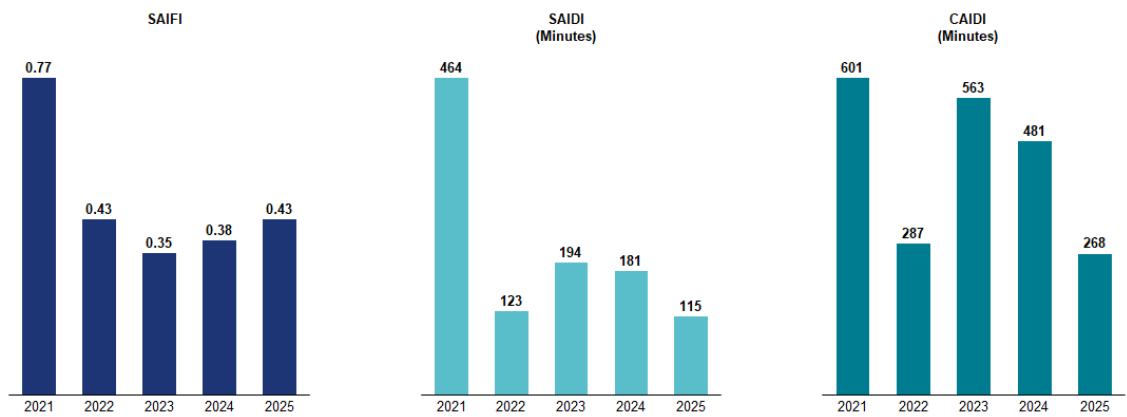
Exhibit 4.41 – DTE Historical Reliability Metrics, Catastrophic Conditions
