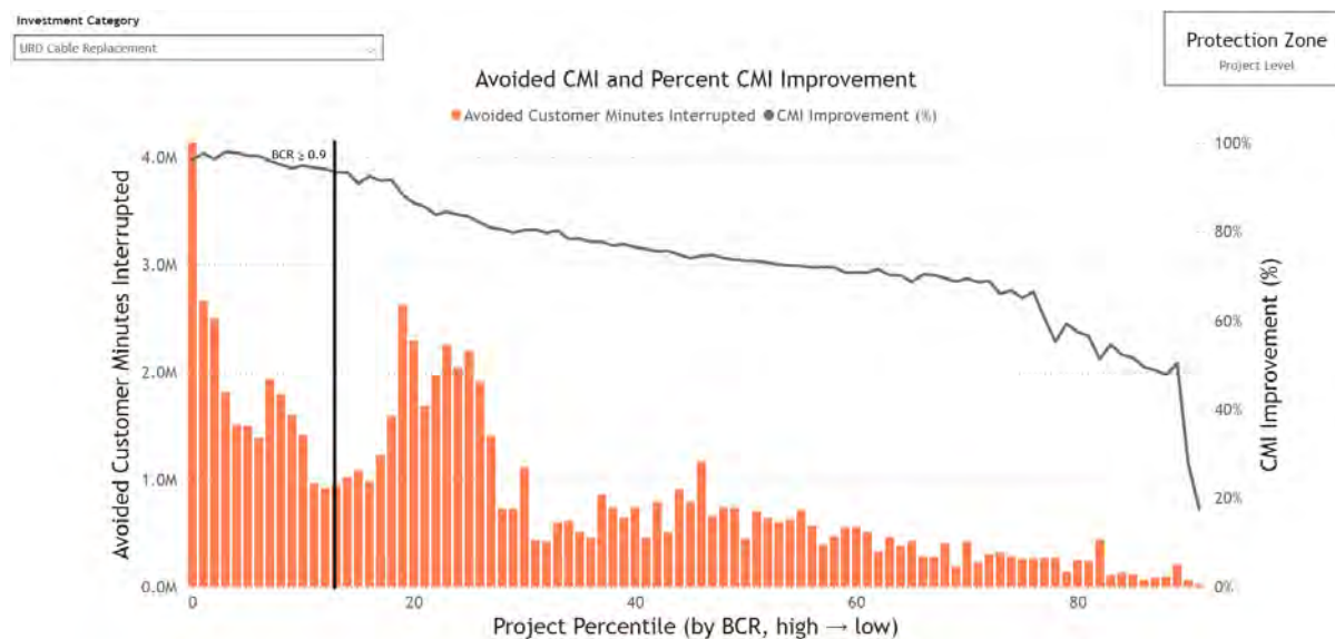
Figure 5-17: URD Replacement Program Avoided Customer Outage Benefit
