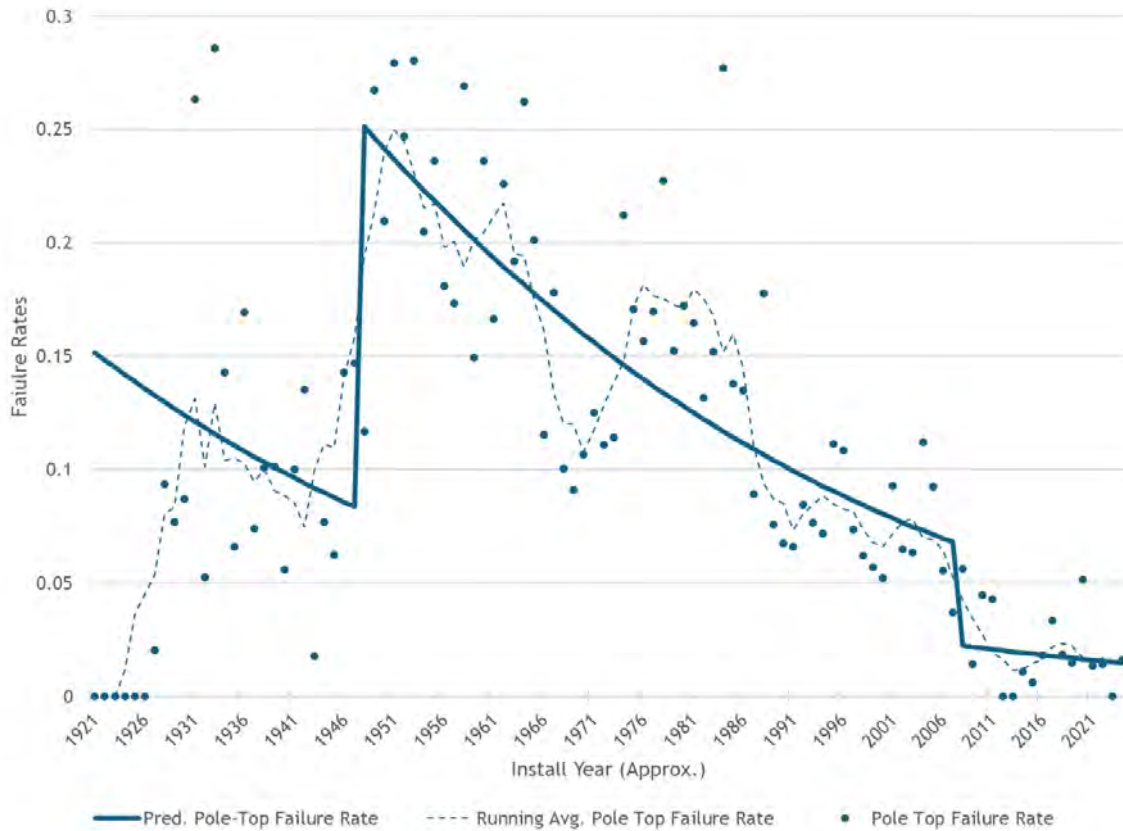
Figure 2-13: Pole Top Predicted Failure Rate
