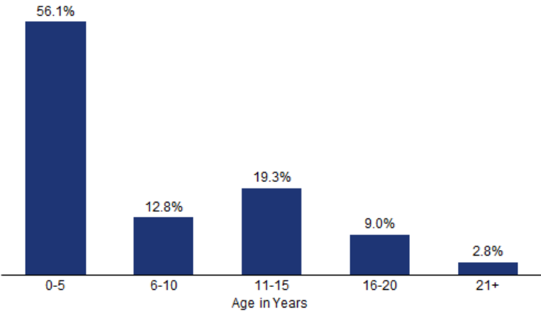
Exhibit 4.20 – Three-Phase Recloser Age Distribution
