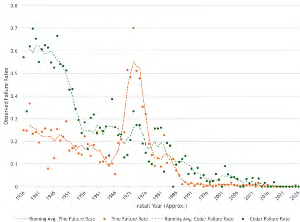
Figure 2-9: Groundline Inspection Failure Rates
