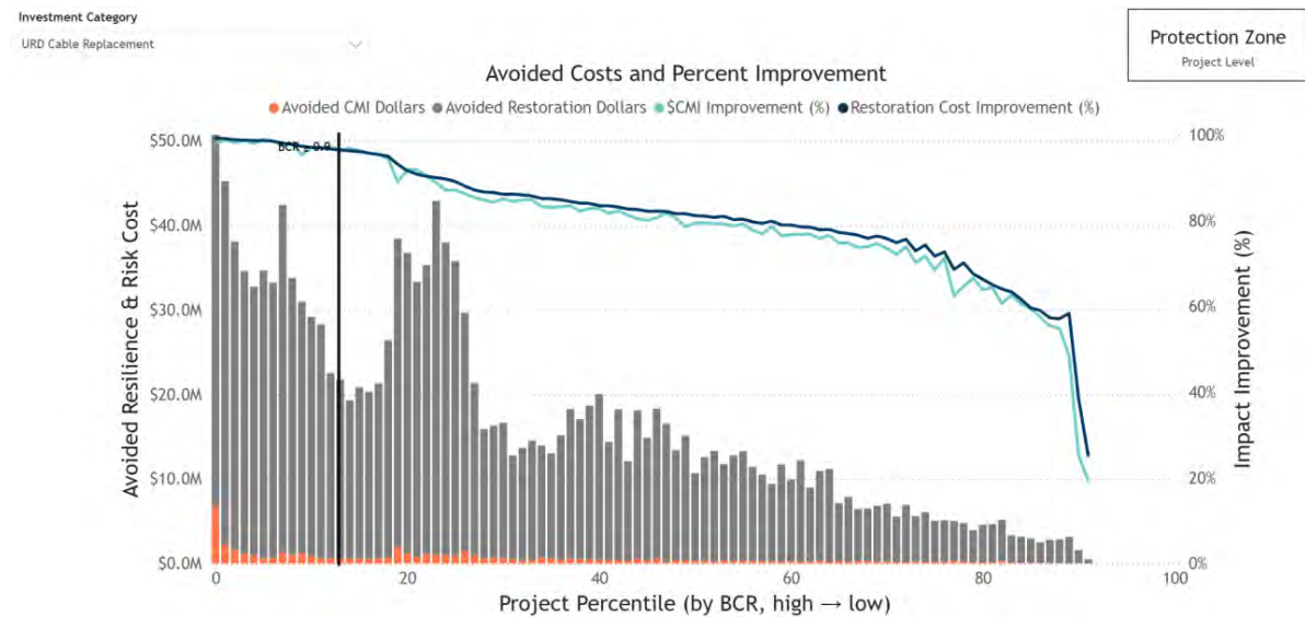
Figure 5-18: URD Replacement Program Benefits Summary
