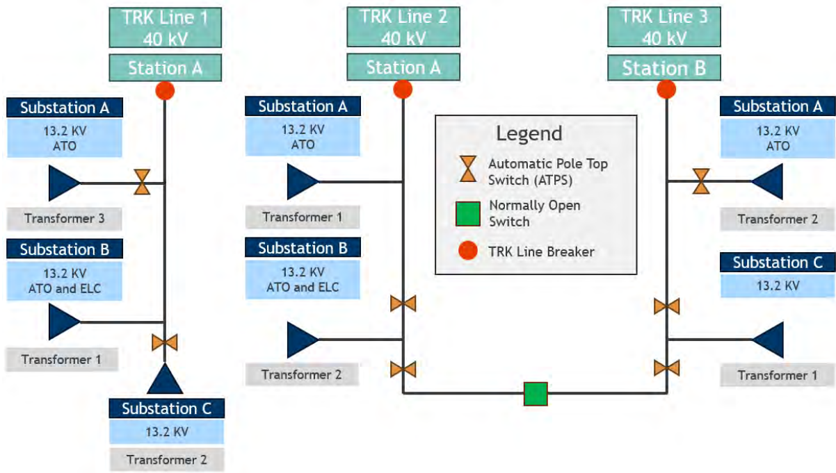
Figure 5-23: Example Trunk Line Configuration
