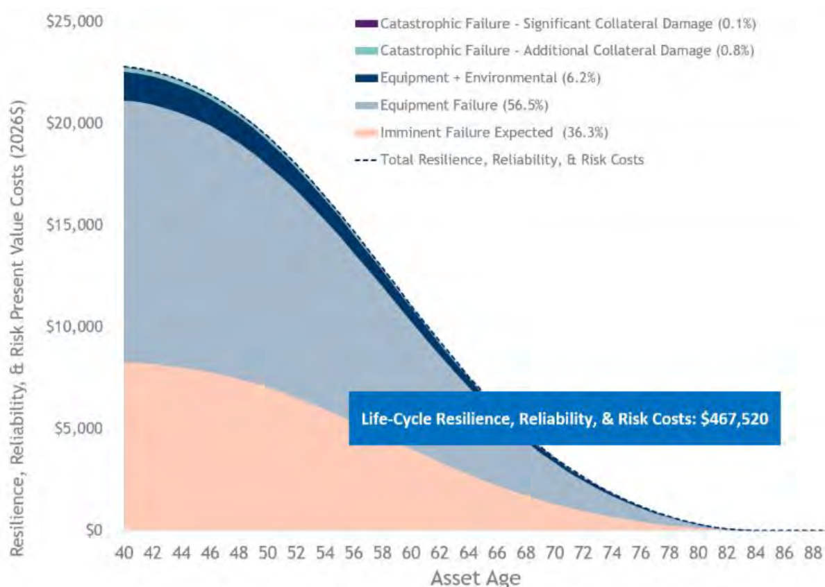
Figure 4-17: Status Quo Total Costs Profile - 40-Year-Old Oil Distribution Breaker [Present Value $]
