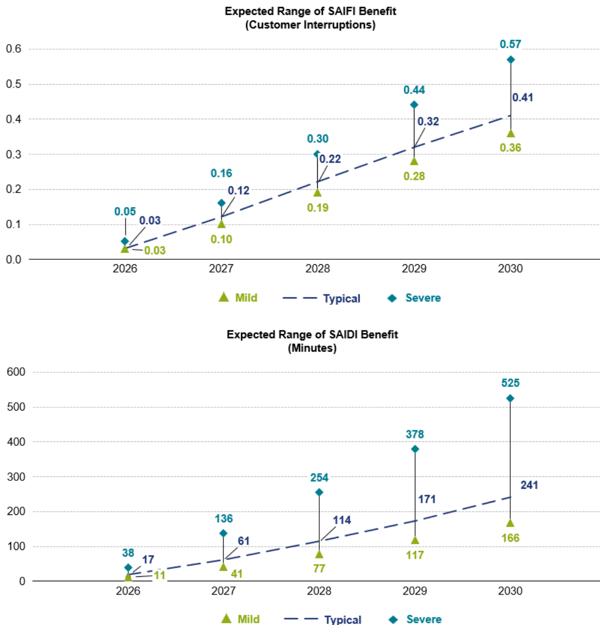
Exhibit 5.25 – Cumulative Reliability Benefits of DSP Investments (For All-Weather Conditions Across Three Weather Scenarios)
