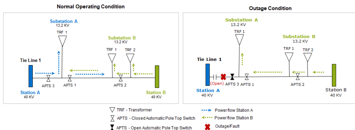
Exhibit 6.61 – Tie Line Configuration with Additional APTS
