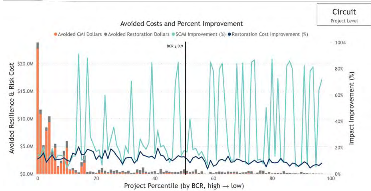
Figure 5-11: Subtransmission PTMM Pole Top Program Benefits Summary
