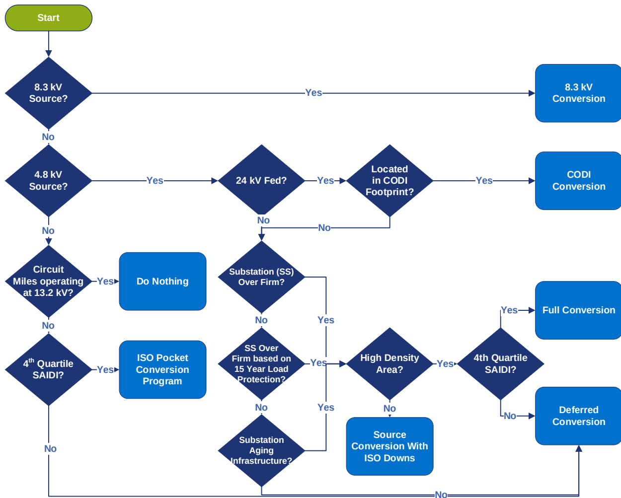
Exhibit 6.38 – Decision Tree for 4.8 kV and 8.3 kV Conversion Tiers
