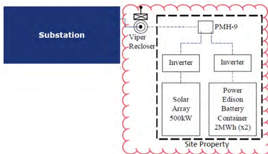
Exhibit 6.52 – Port Austin NWA Solution
