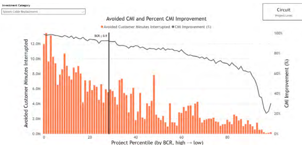
Figure 5-20: System Cable Program Avoided Customer Outage Benefit
