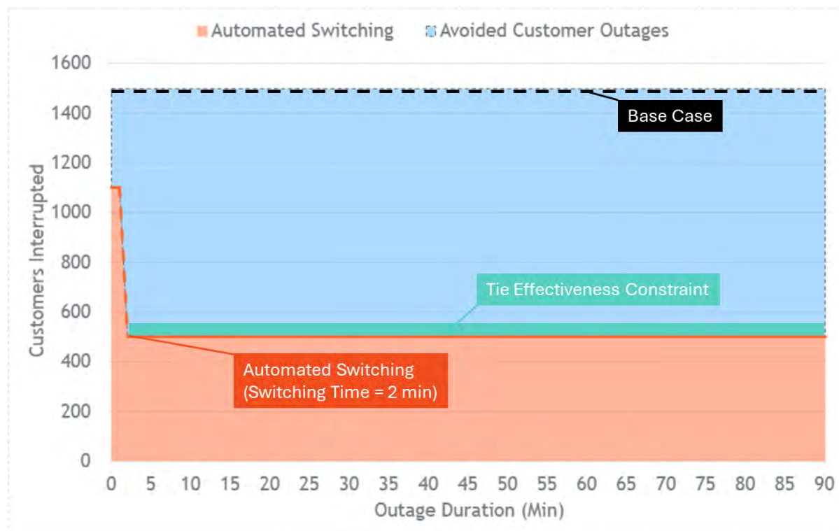
Figure 4-27: Mainline Outage Profile with Sectionalization and Automated Tie
