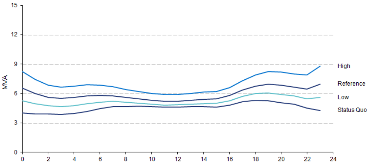
Exhibit 5.4 – Winter Peak Day Example
