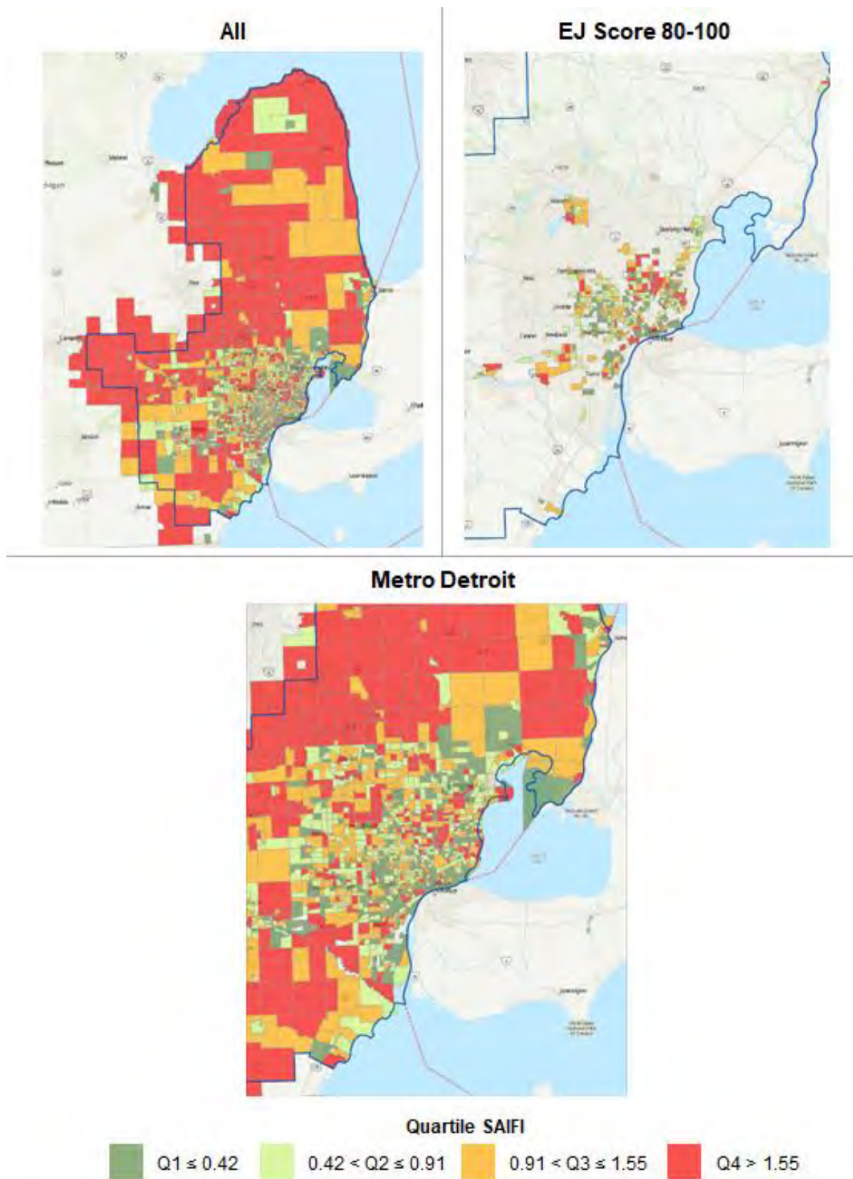
Exhibit 4.63 – 2025 All-Weather SAIFI by Census Tracts in DTE’s Service Area
