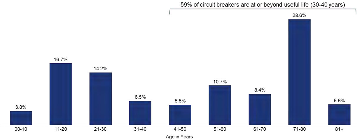
Exhibit 4.14 – Circuit Breaker Age Distribution
