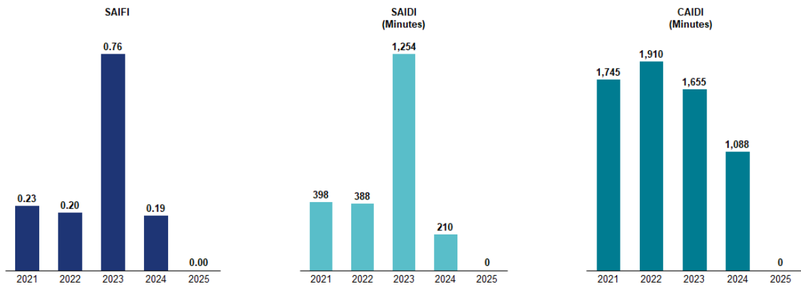
Exhibit 4.41 – DTE Historical Reliability Metrics, Catastrophic Conditions
