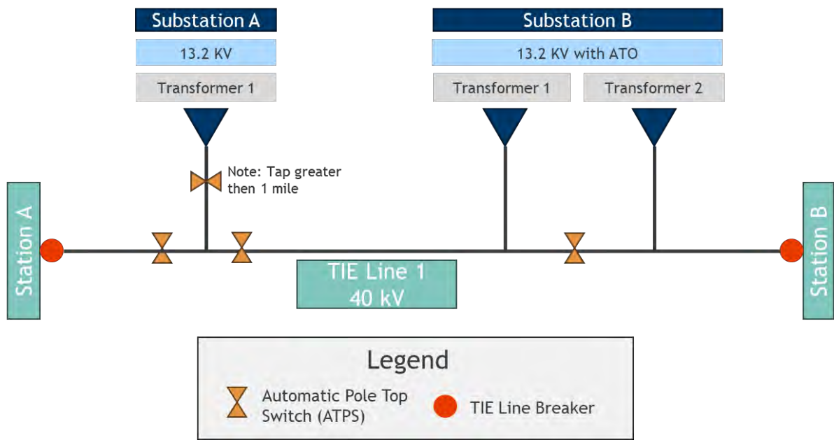
Figure 5-24: Example Tie Line Configuration
