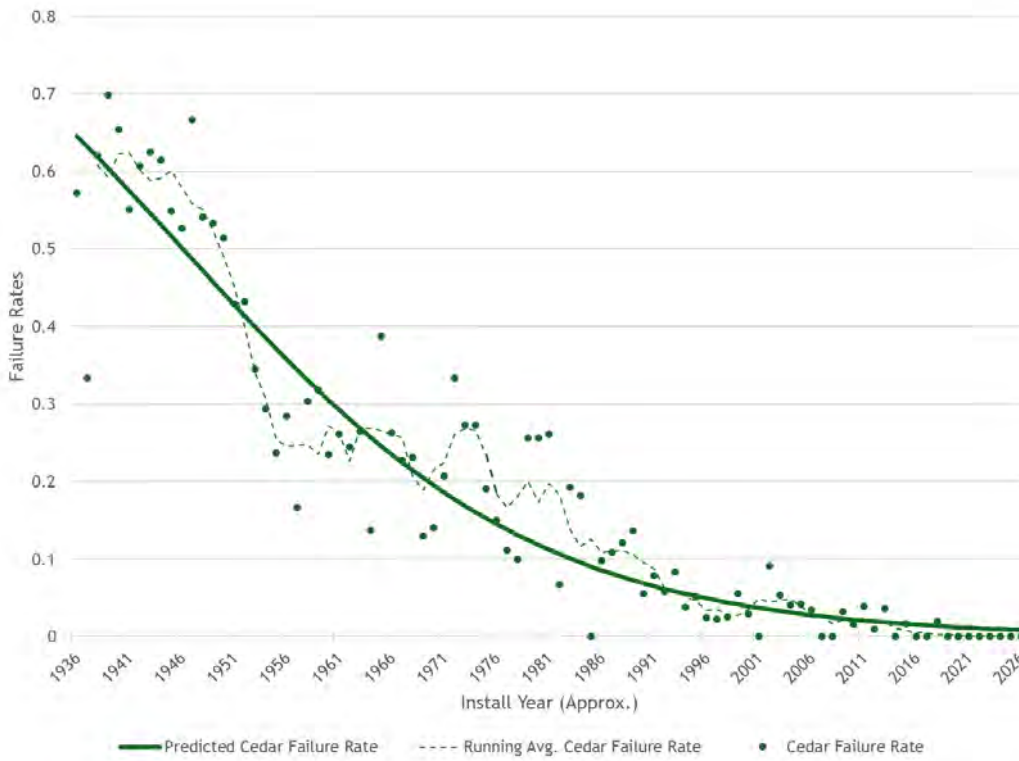
Figure 2-11: Cedar Pole Predicted Failure Rate
