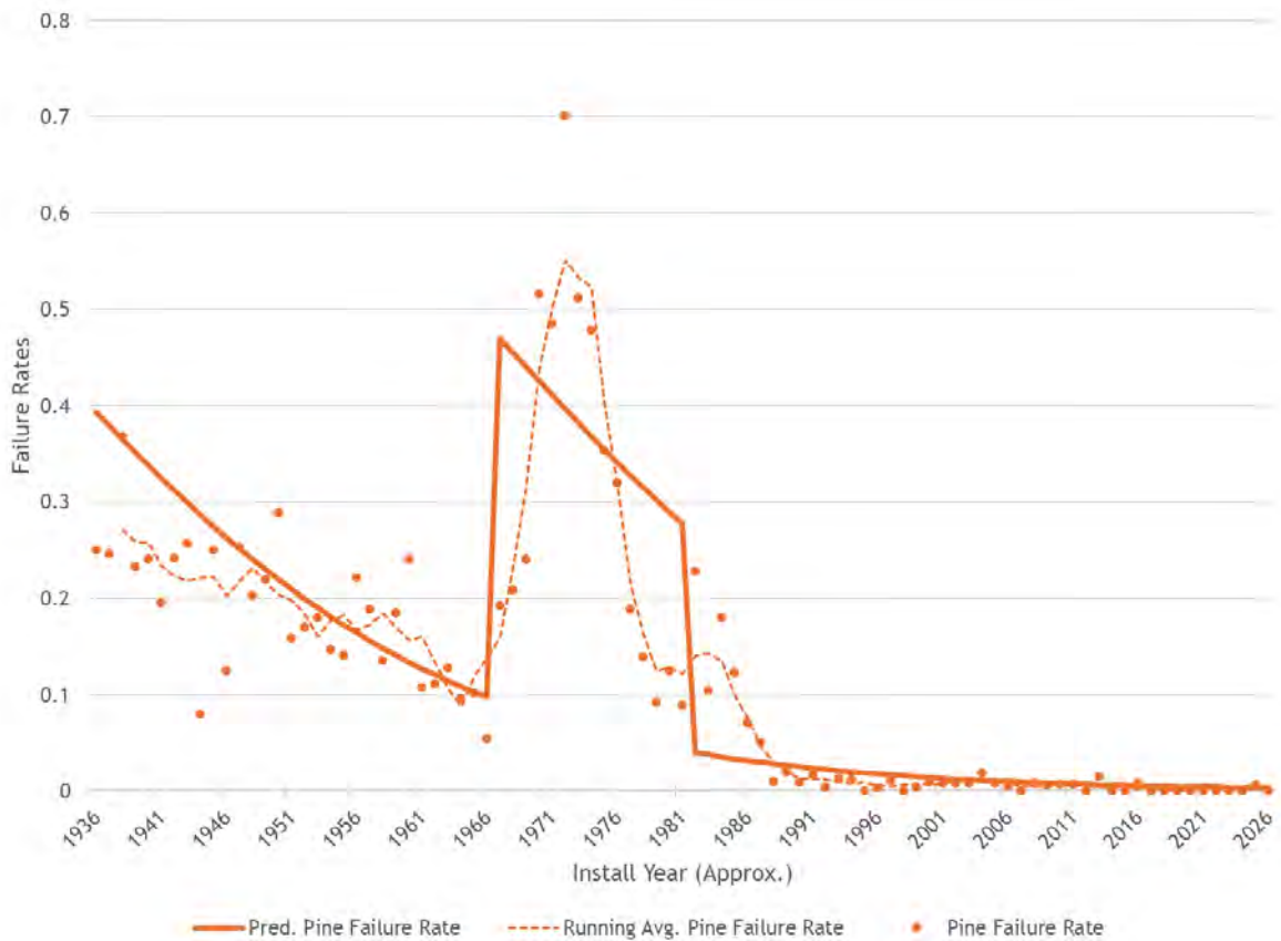
Figure 2-12: Pine Pole Predicted Failure Rate
