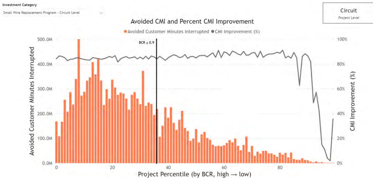
Figure 5-13: Small Wire Replacement Program Avoided Customer Outage Benefit
