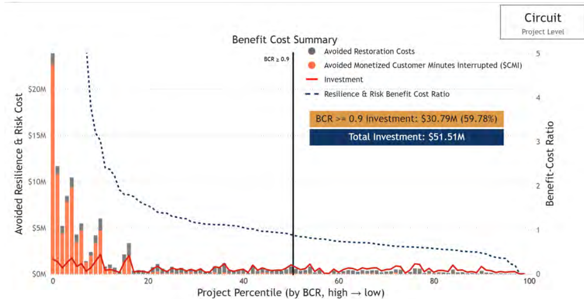
Figure 5-12: Subtransmission PTMM Pole Top Inspection Program BCR Summary
