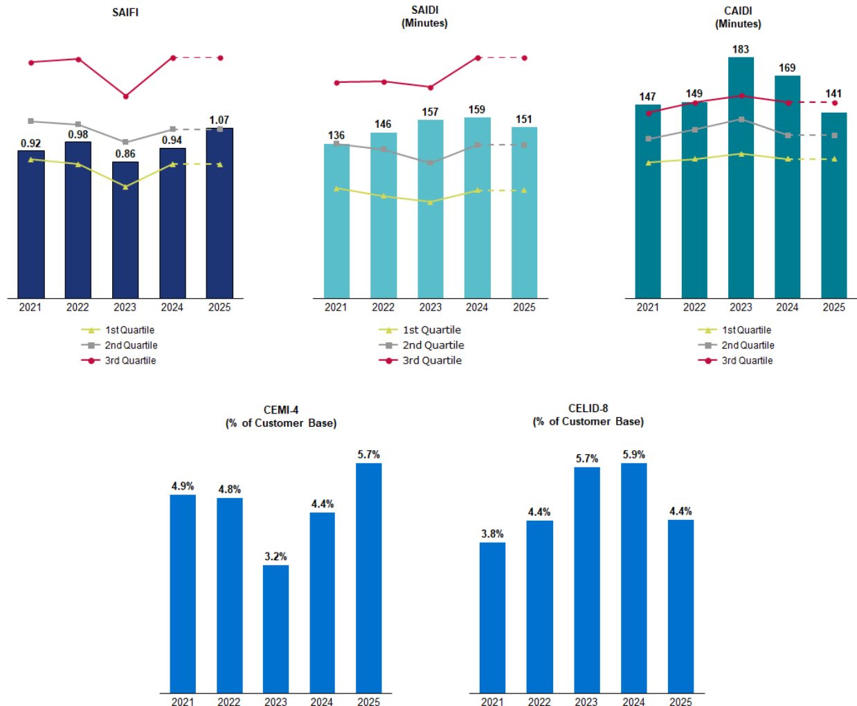
Exhibit 4.38 – DTE exMED Reliability Metrics 52
