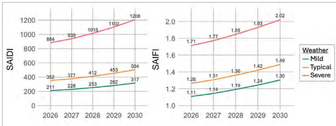
Figure 7. Forecast SAIDI and SAIFI by weather scenario given zero-investment scenario
