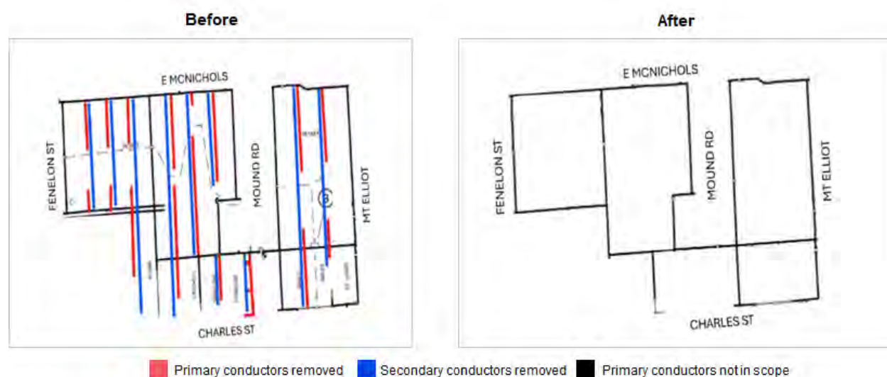
Exhibit 6.23 – DC 1136 St. Louis Circuit Topology
