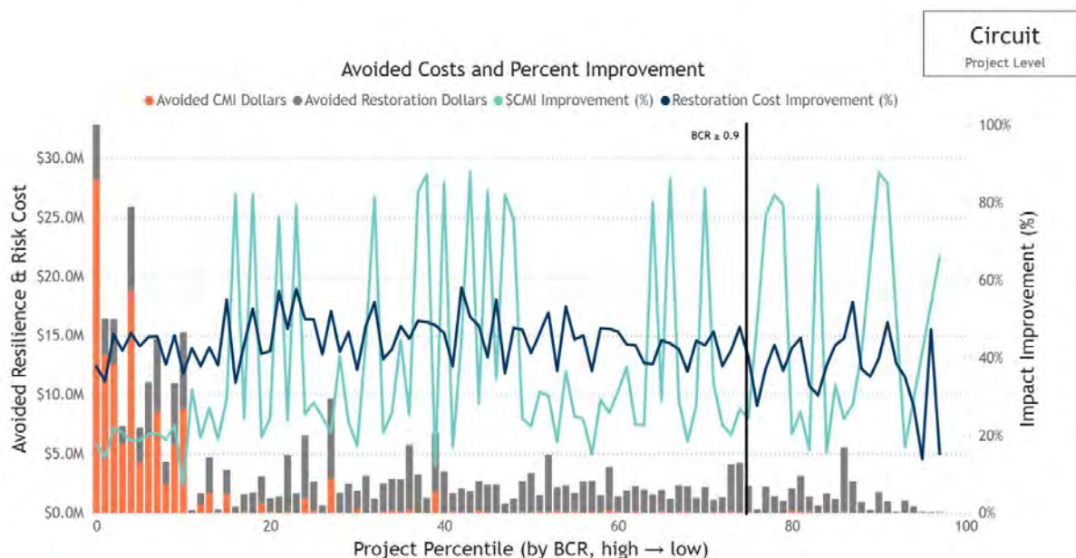
Figure 5-8: Subtransmission PTMM Groundline Inspection Program Benefits Summary
