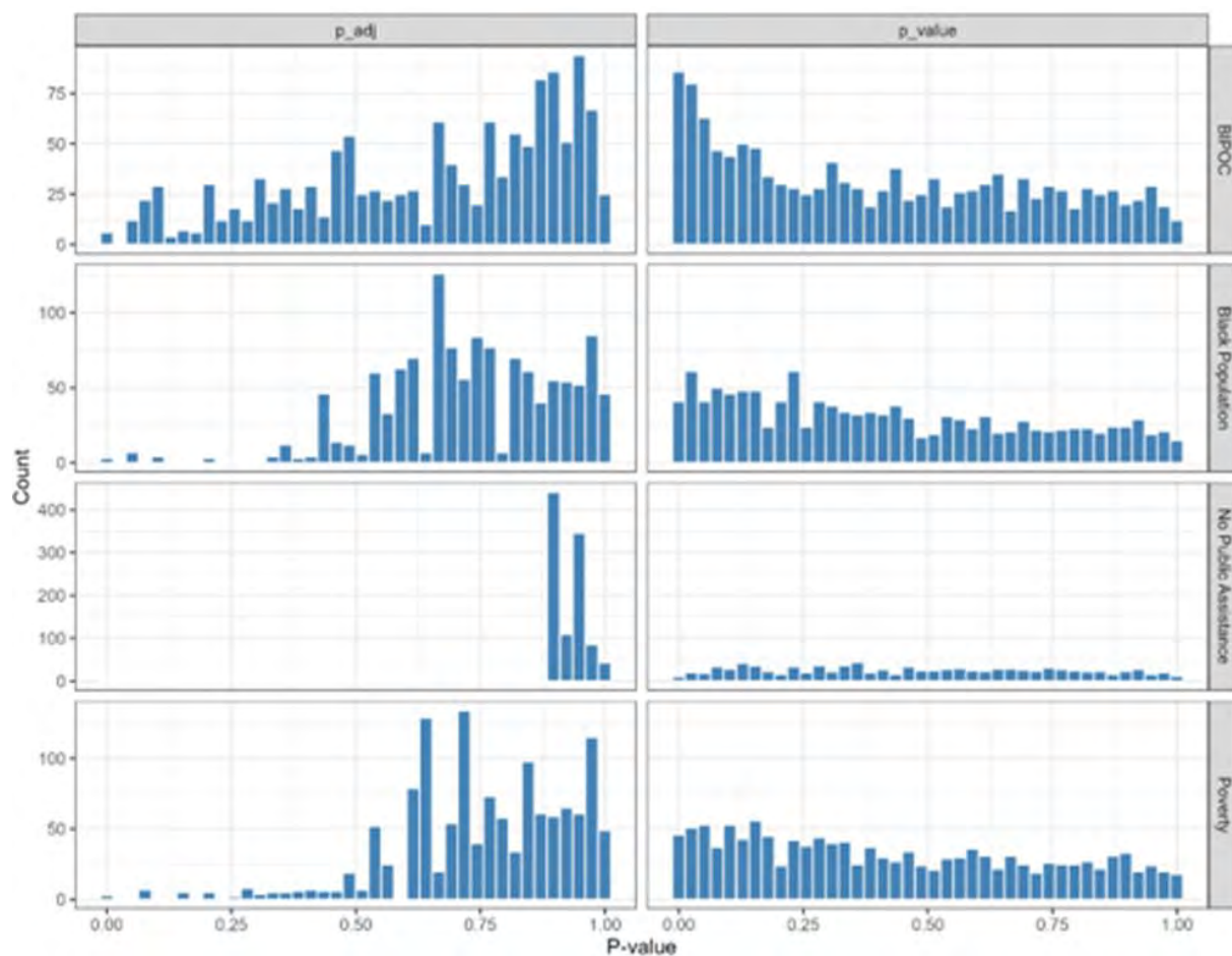
Exhibit 8.32 – Distribution of Raw and FDR-Adjusted P-Values
