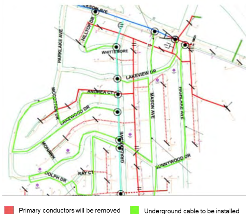
Exhibit 6.24 – DC 9836 Spruce Circuit Scope
