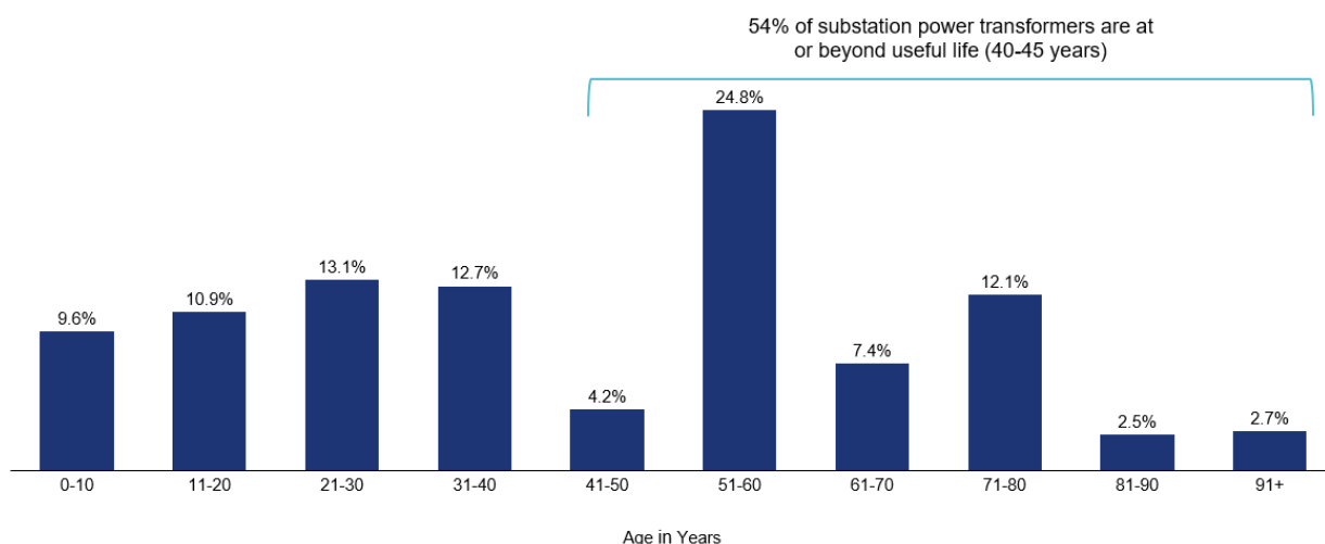
Exhibit 4.10 – Substation Power Transformer Age Distribution
