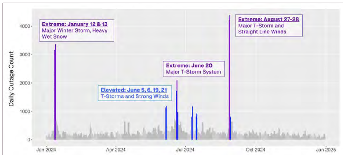
Figure 2. Sample of identified elevated or extreme weather days based on daily outage counts
