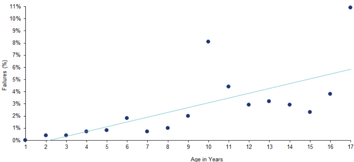
Exhibit 6.93 – Legacy Meter Failure Rate by Meter Age
