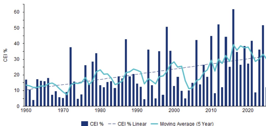
Exhibit 2.4 – Upper Midwest Climate Extremes Index 16
