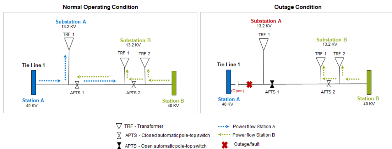
Exhibit 6.60 – Tie Line Configuration, Baseline APTS
